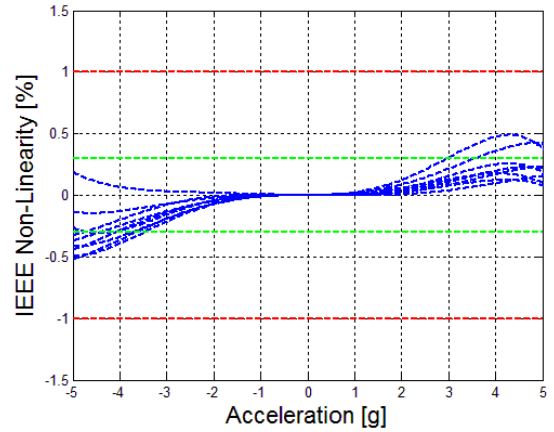
Figure 22 : Non-linearity IEEE
