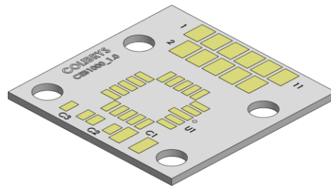
Figure 48 : Ceramic Evaluation Board (CEB1000_1) for LCC20. Dimension: 25mm x 25mm
