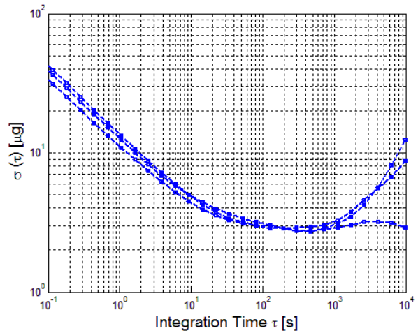
Figure 26: Allan Variance
